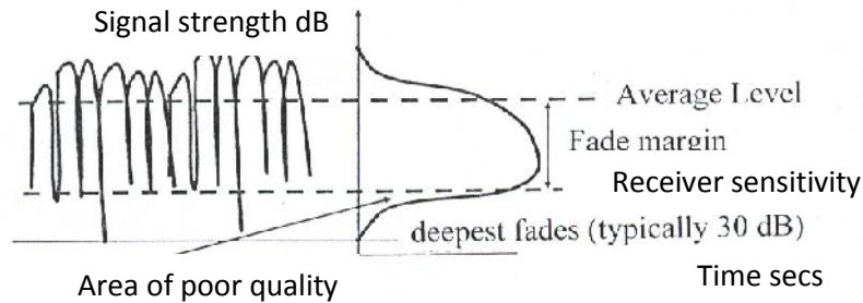
Figure 3: Small scale fading (Rayleigh fading) [9]
