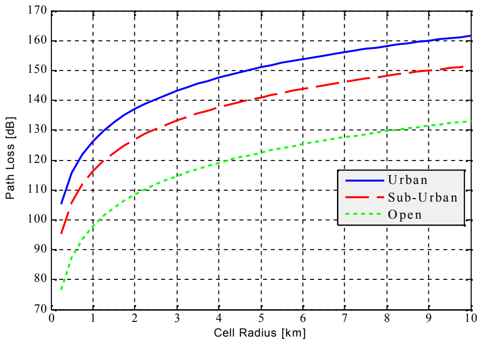
Figure 1: Path Loss as a Function of Cell Radius for Urban , Sub-Urban & Open Area .at f=900\text{MHz} . h(t)=30\text{m} h(r)=1.5\text{m}
